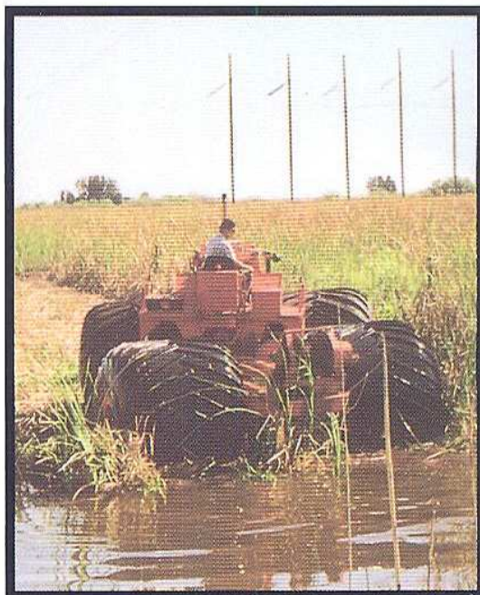
4 X 4 Roughneck with Rolligon 72 X 68 Tires
